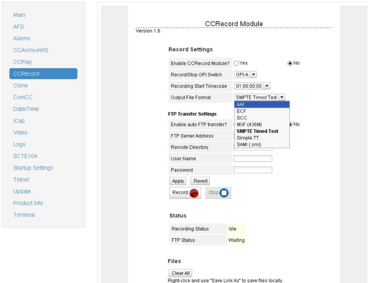
Figure 1: CCRRecord Interface Showing Supported File Formats
